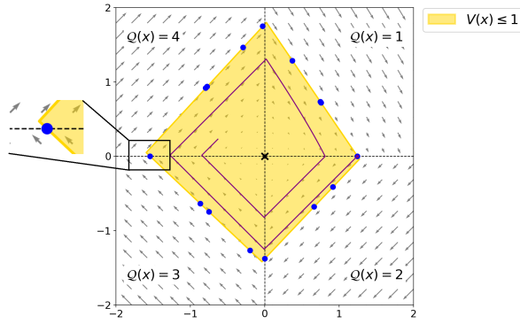
Fig. 3. 4-piece polyhedral Lyapunov function V for the system in Example 1. The blue dots are the states involved in the constraints leading to this polyhedral function. A sample trajectory starting from x = [1.25, 0]^T is represented in purple. Note the small “offset” (see zoomed-in inset): the domains of the linear pieces of V do not coincide with the domains of the hybrid system; this is necessary for condition (C2) in Proposition 1 to be satisfied at the boundary of these domains.
