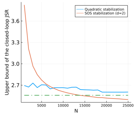
Fig. 3. Comparison of quadratic stabilization and SOS stabilization: the dashed line is the JSR of the white-box quadratic stabilization solution.
