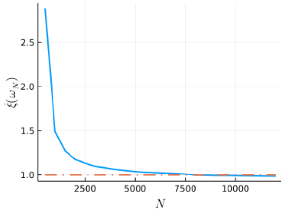
Fig. 5. Feasibility measure of the LQR solution
